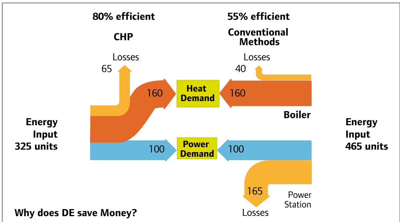
CHP is a more efficient way of meeting local electricity and heating demands compared with the traditional approach of inputting electricity from centralised power stations and the use of local gas-fired boilers.
