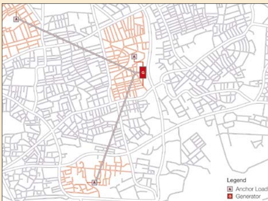
Type 2 Multi-site, mixed-use schemes
