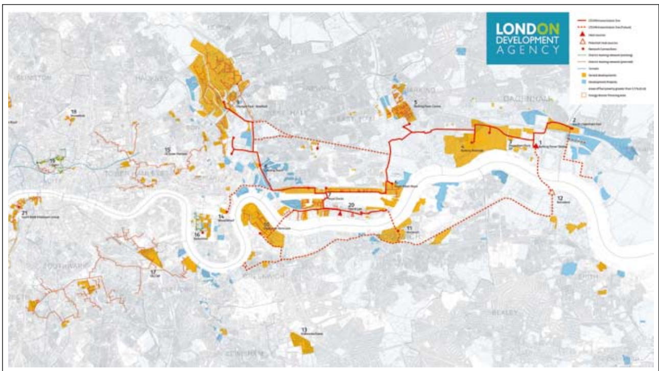
Proposed London Thames Gateway Heat Network
